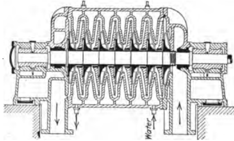
FIG. 86.—Original Rateau turbine blower.
